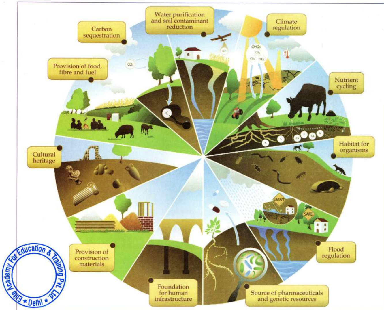
Figure 1: Schematic diagram of soil functions
